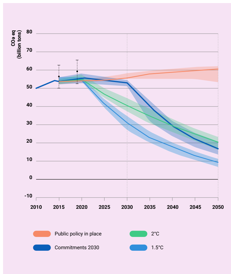
Figure 9: Projected global GHG emissions over 2015–2050 based on current policies and commitments by countries. Source: Adapted from chart produced by Dr. Valérie Masson-Delmotte. 30
