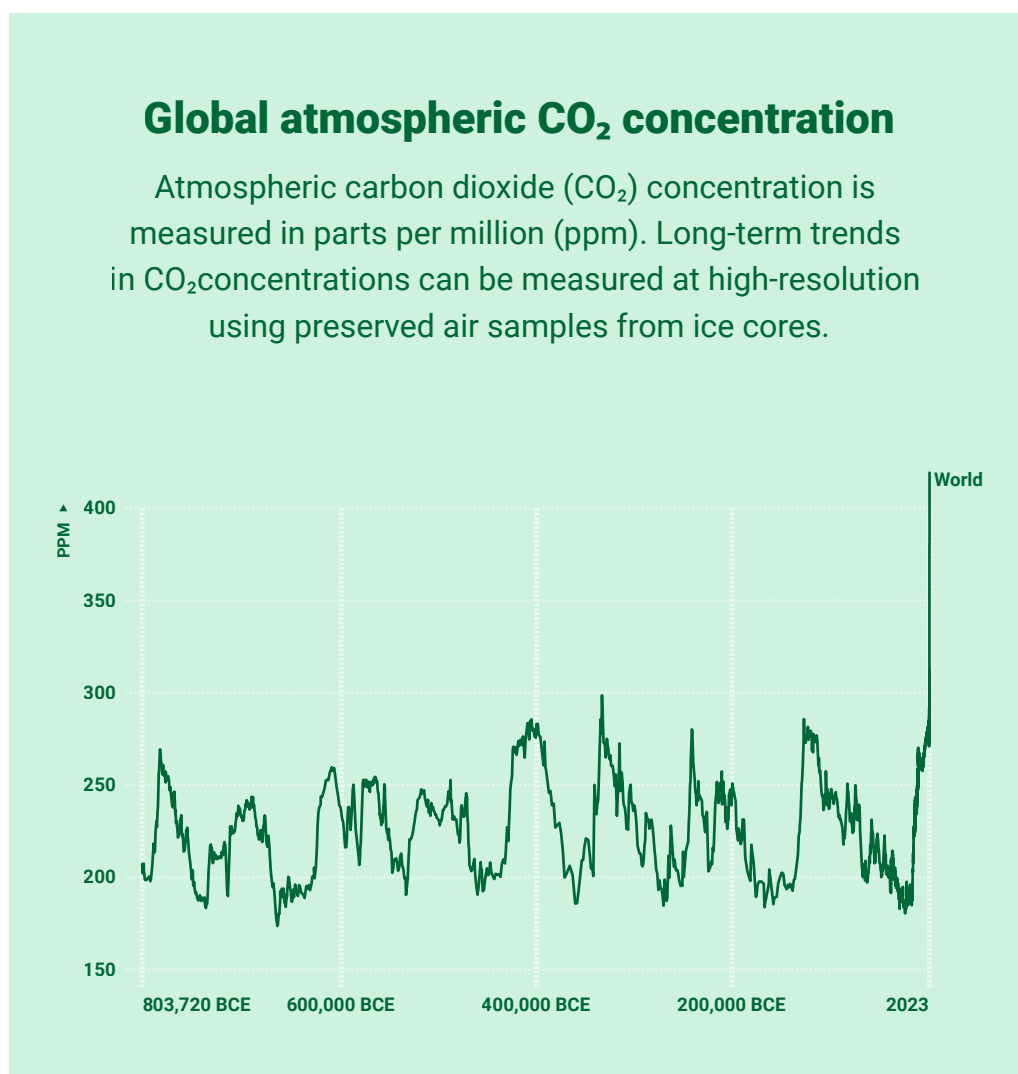
Figure 3: Concentration of carbon dioxide in the atmosphere for the past 800,000 years. (BCE stands for Before the Common Era). Source: Ritchie et al., 2020. 11
